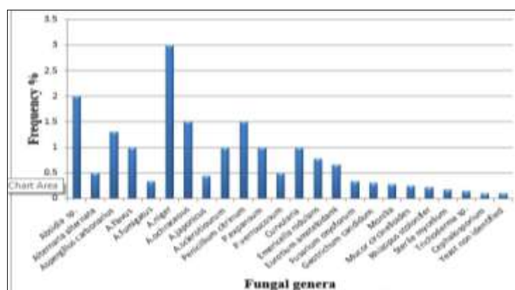
Figure 3: Frequency (%) of fungal genera on DRBC.PDA and MEA medium.
