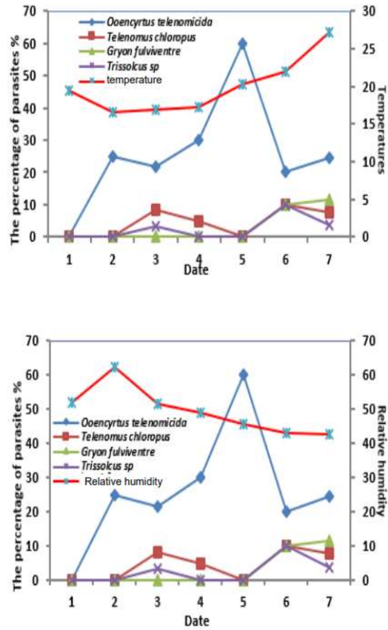
Figure-3- The relationship between temperature and relative humidity and the seasonal spread of sunn pest egg parasitoids in Najaf/Kufa in 2019
