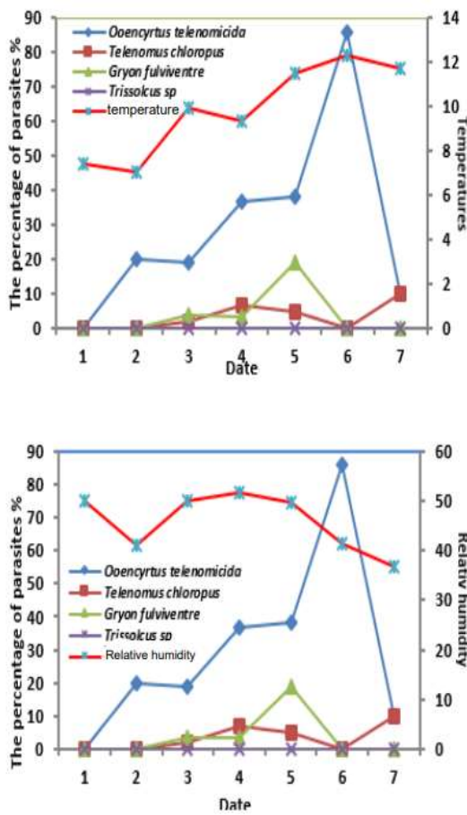
Figure-4- The relationship between temperature and relative humidity and the seasonal spread of sunn pest egg parasitoids in Najaf/Kufa in 2020
